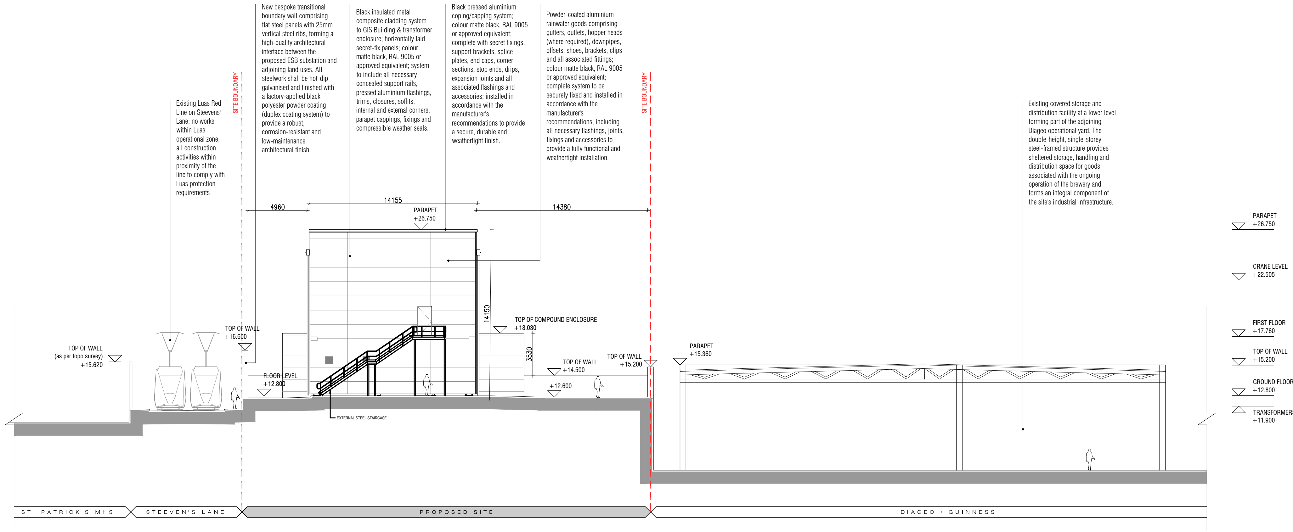
PROPOSED CONTIGUOUS SOUTH SECTIONAL ELEVATION scale 1:200 at A1
